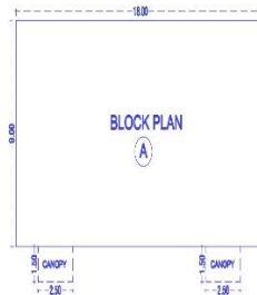
BLOCK PLAN
