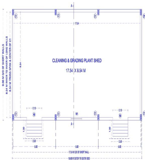
CLEANING & GRADING PLANT SHED PLAN
